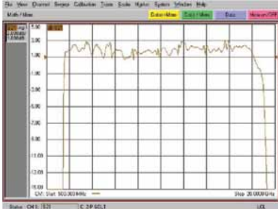
Fig 1. S21, all channels 'ON'
