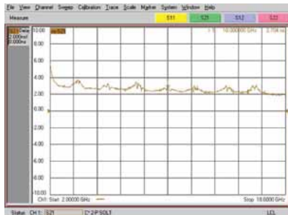
Fig 4. Full band Group Delay response
