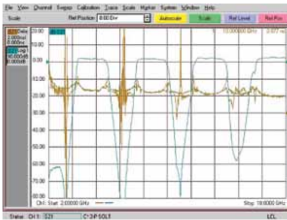
Fig 5 & 6. Group Delay response in 'On' and 'Off' Bands.
