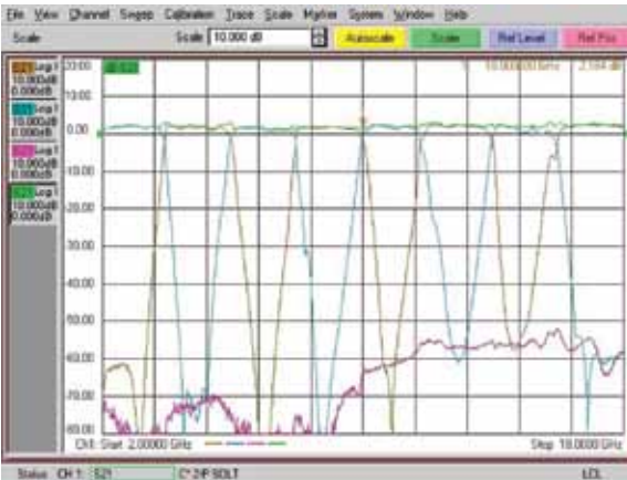
Fig 3. Overlay of individual channels
